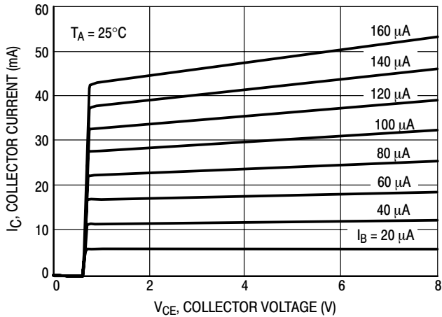
Figure 1. I_C - V_{CE}
