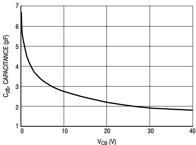
Figure 6. Capacitance
